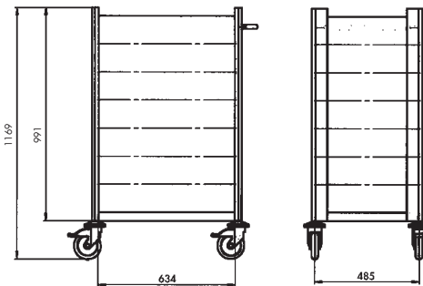
Case for 7 height grids
