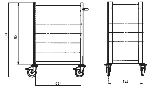
Case for 6 height grids
