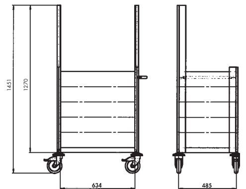
Case for 5 height grids with extended profile supports at rear
