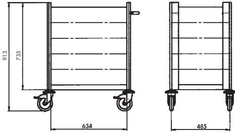
Case for 5 height grids
